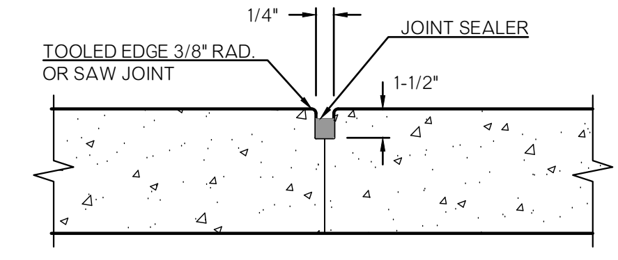
CONTRACTION JOINT NO SCALE
