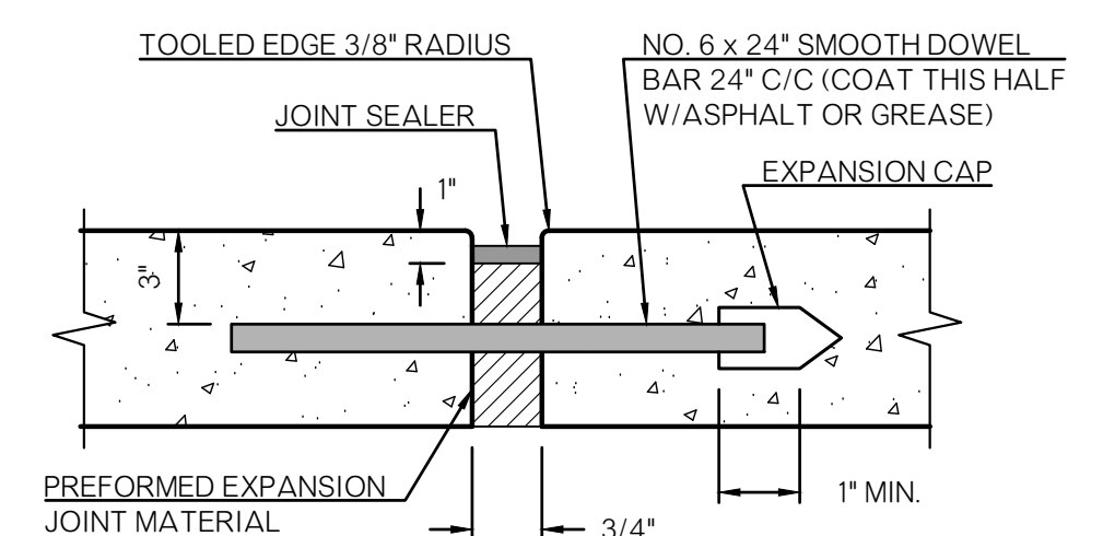
EXPANSION JOINT NO SCALE
