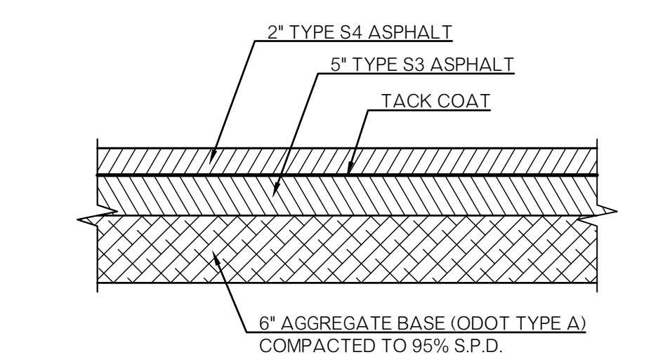
HEAVY DUTY ASPHALT PAVING SECTION NO SCALE
