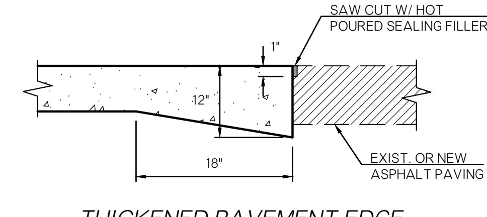
THICKENED PAVEMENT EDGE (TYPICAL AT CONCRETE & ASPHALT JOINT)
