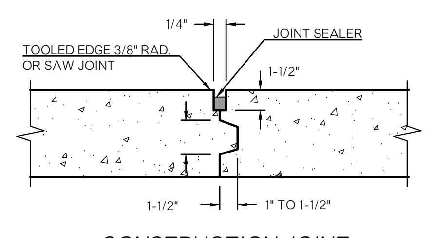
CONSTRUCTION JOINT NO SCALE
