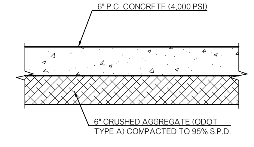
P.C. CONCRETE PAVING SECTION
