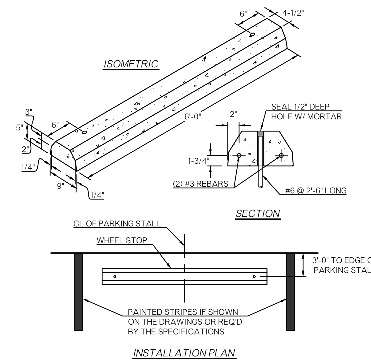
PRECAST CONCRETE WHEEL STOP DETAILS NO SCALE
