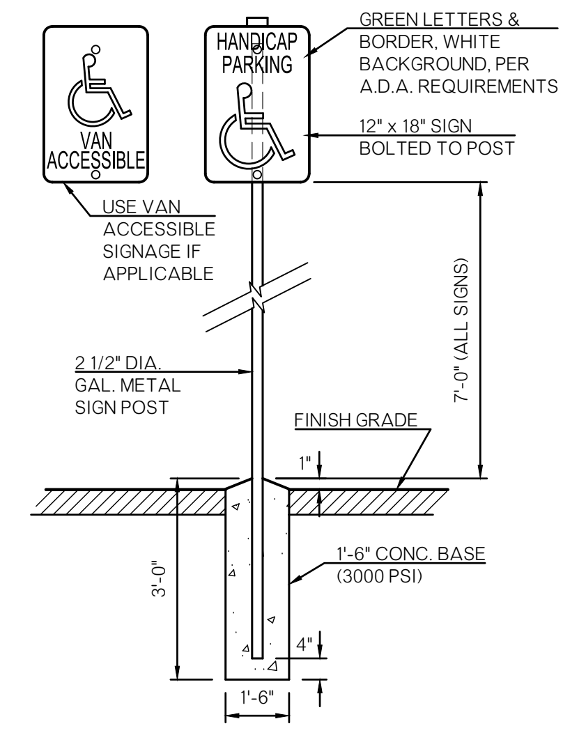
HANDICAP SIGN DETAIL NO SCALE
