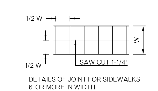
TYPICAL SIDEWALK SECTION NO SCALE
