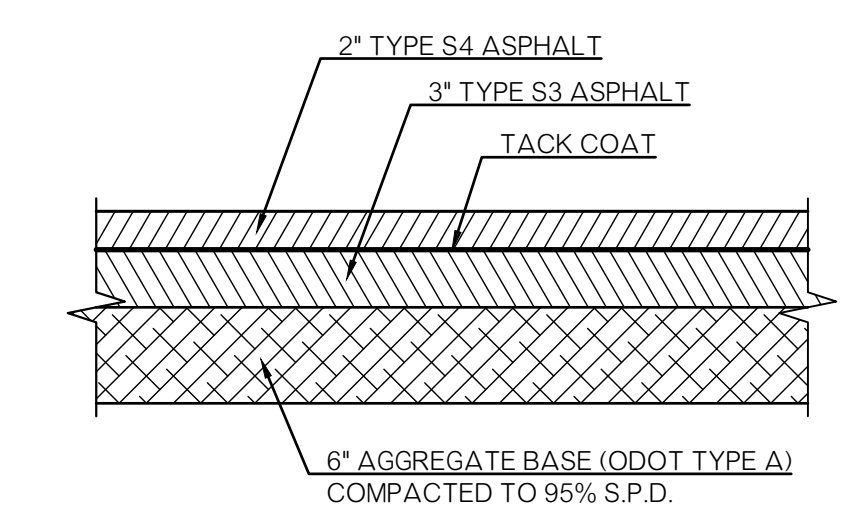
LIGHT DUTY ASPHALT PAVING SECTION NO SCALE
